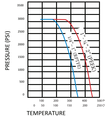
PRESSURE - TEMPERATURE RATING 1/4" - 2"
