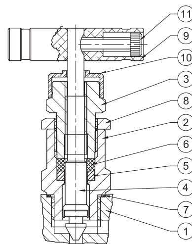
SECTIONAL DETAILS OF VALVE
