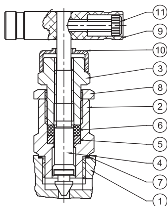
SECTIONAL DETAILS OF VALVE
