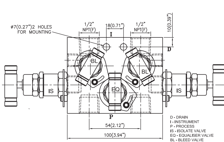
SECTIONAL DETAILS OF VALVE
